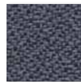
magnetic fabric
