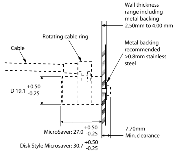
Slot Clearance—Side view All measurements are in millimeters
